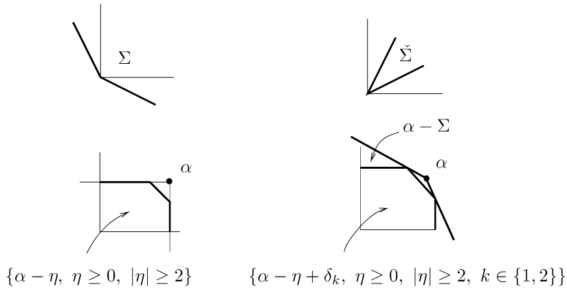
Fig. 1. Cone \Sigma and related sets in dimension 2.
