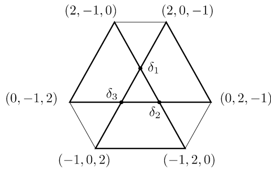
Fig. 2. Trace of \Sigma (convex hull) and of \{\eta - \delta_k, \eta \geq 0, |\eta| \geq 2, k \in \{1, 2, 3\}\} (union of three triangles) on the hyperplane \{x_1 + x_2 + x_3 = 1\} of \mathbb{R}^3 .
