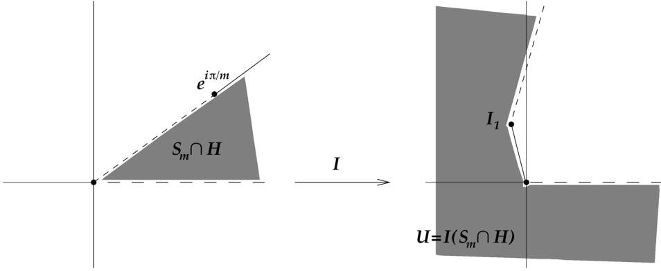
FIG. 2. Domain \mathcal{S}_m \cap \mathbb{H} and its image by I .
